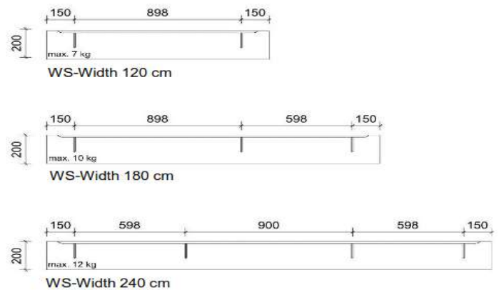
Figure 2: wallboard sizes and position of suspension units
