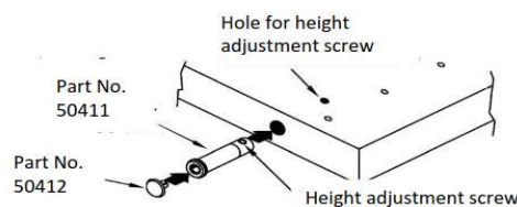
Fig. 2: Height adjuster assembly
