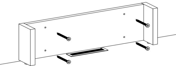
Fig. 4: Wall mounting
