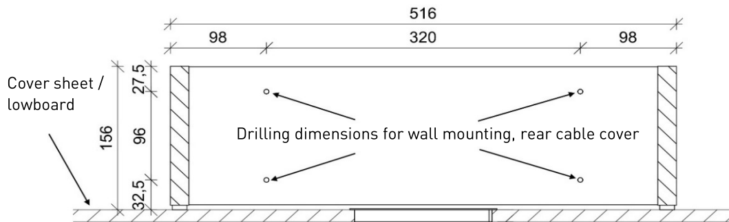
Fig. 3: Drilling dimensions
